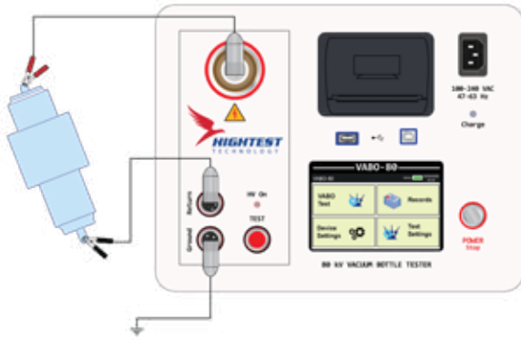
Illustration: Circuit Breaker Vacuum Bottle Testing with VABO-80
